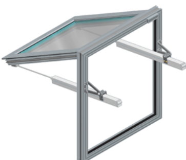
Fig.43 - mcr OSO THERM 75 smoke exhaust window with two G spindle actuators with shifted pivot point
