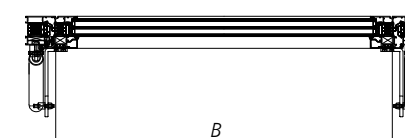
Fig.67 - B-B horizontal cross-section through mcr OSO THERM 75 smoke exhaust window in closed position
