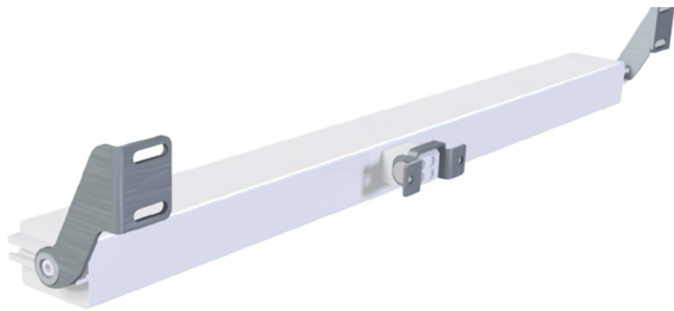
Fig.113 - HCV chain actuator with consoles for outward opening window
