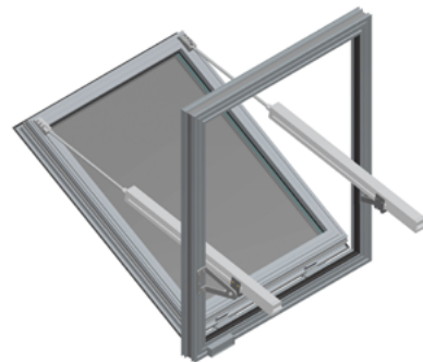
Fig.39 - mcr OSO THERM 75 smoke exhaust window with two G spindle actuators with shifted pivot point
