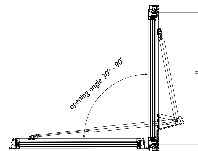
Fig.19 - A-A vertical cross-section through mcr OSO THERM 75 smoke exhaust window in open position
