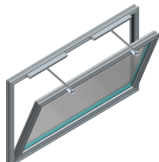
Fig.54 - mcr OSO THERM 75 smoke exhaust window with two HCV chain actuators
