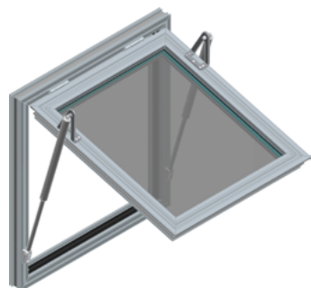
Fig.55 - mcr OSO THERM 75 smoke exhaust window with two S spindle actuators
