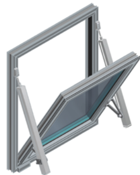
Fig.86 - mcr OSO THERM 75 smoke exhaust window with two G spindle actuators with shifted pivot point
