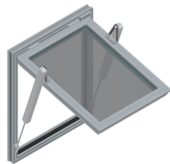
Fig.88 - mcr OSO THERM 75 smoke exhaust window with two G spindle actuators
